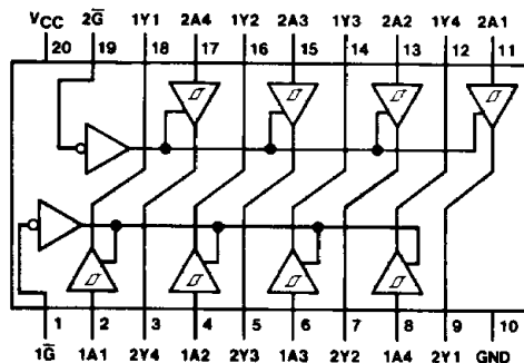
Dual-In-Line Package
